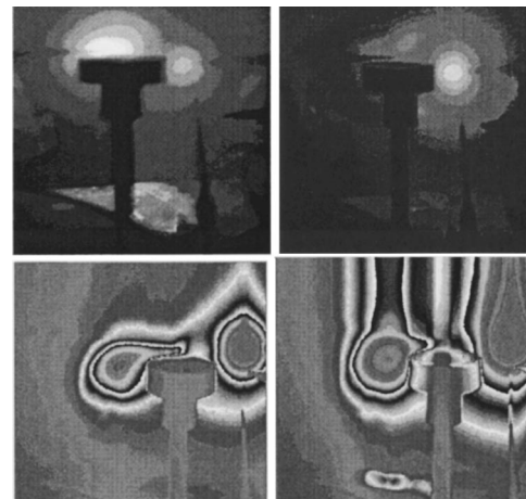
FIG. 3. First and second panel show ion and electron injection, respectively, revealing magnetic trapping of plasma. Third and fourth panels show electron injection at 2.5 kV and 4 kV, respectively, in false color.
