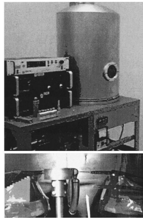
FIG. 2. The outside of the 19 inch stainless bell jar vacuum chamber (top panel) and the inside of the UAH Spinning Terrella Accelerator. See text for details.
